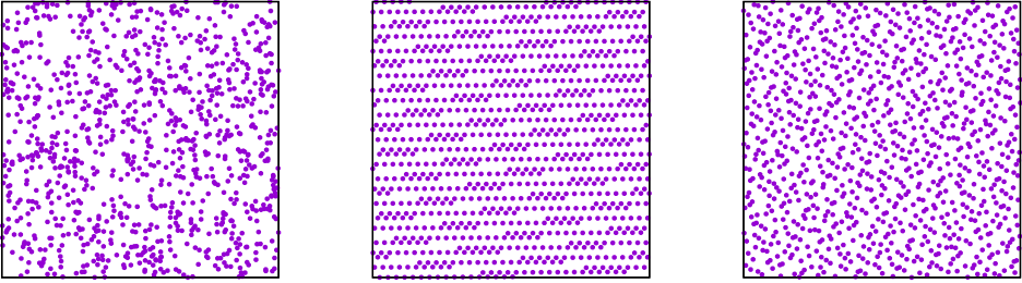
Figure 2: Typical distributions of pseudo-random points (left), and quasi-random low-discrepancy points: additive (center) and base-2/3 Halton (right) sequences. The first thousand points are plotted in each case.
